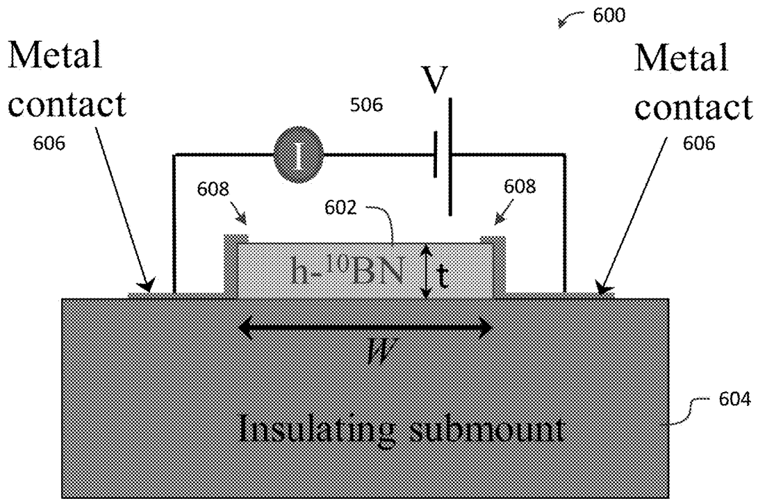
Cross-sectional view
