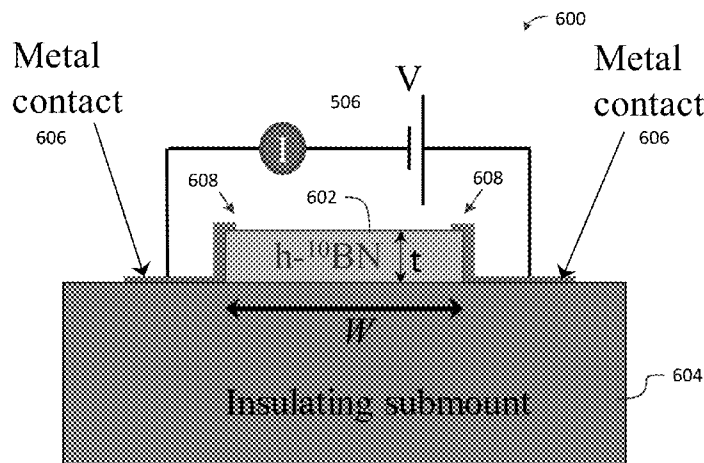
Cross-sectional view
